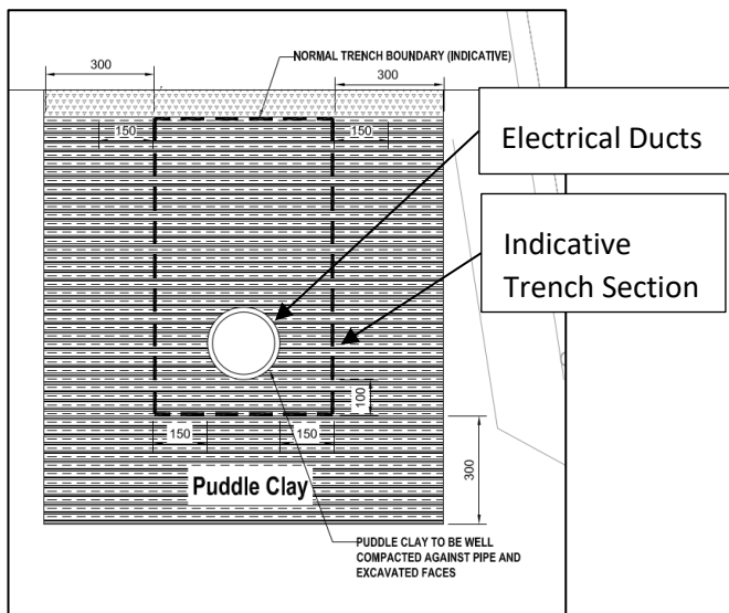
Plate 6.10 Spaced puddle clay stanks along the cable route in the areas prone to groundwater risk
